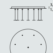
MINERVA R07 ROSONE A 7 LUCI CON DRIVER 220/240Vac 50-60 Hz 7-LIGHT CANOPY WITH DRIVER 220/240Vac 50-60 Hz
