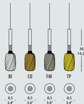
MINERVA SS 6,1W 785 Lm 2700K Cri>80 24Vdc LED CE F IP 20 EAC
