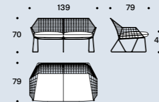
Divano / Sofa
