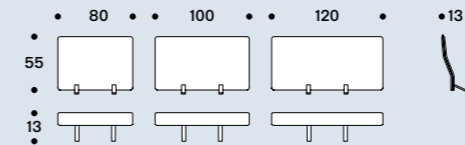
Schienali / Backrests
