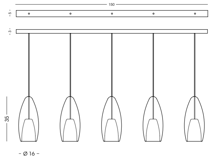
GIG1397.150.5L Binario a soffitto / Ceiling track vetro/glass Ø16 cm - cavo/cable 150 cm 5 E27 x max 105W 220-240V CE IP20 (1m)
