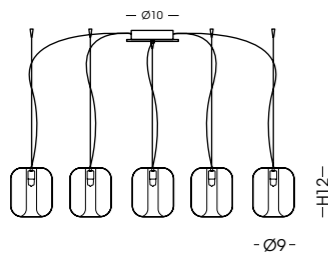
743.5L Sospensione / Hanging lamp vetro/glass Ø9 cm - cavo/cable 250 cm 5 G9 x max 42W 230V CE IP20 1m
