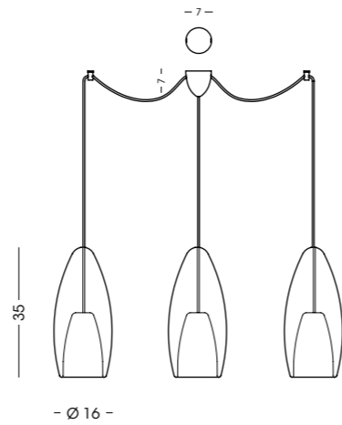
GIG1393.3L Sospensione / Hanging lamp vetro/glass Ø16 cm - cavo/cable 250 cm 3 E27 x max 105W 220-240V CE IP20 (1m)
