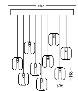
744.9L Plafoniera / Ceiling lamp vetro/glass Ø6 cm - cavo/cable 150 cm 9 G9 x max 42W 230V CE IP20 1m
