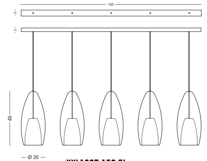
XXL1397.150.5L Binario a soffitto / Ceiling track vetro/glass Ø20 cm - cavo/cable 150 cm 5 E27 x max 105W 220-240V CE IP20 (1m)
