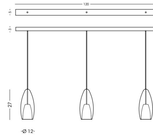
1397.120.3L Binario a soffitto / Ceiling track vetro/glass Ø12 cm - cavo/cable 150 cm 3 E14 x max 60W 220-240V CE IP20 (1m)
