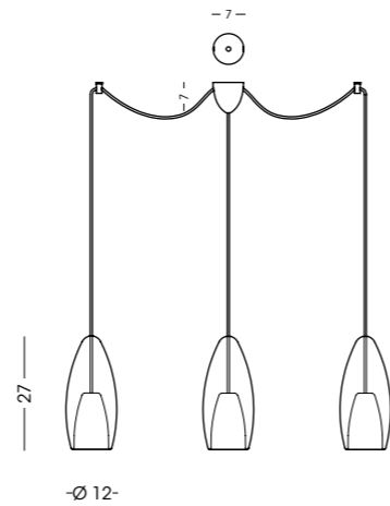
1393.3L Sospensione / Hanging lamp vetro/glass Ø12 cm - cavo/cable 250 cm 3 E14 x max 60W 220-240V CE IP20 (1m)
