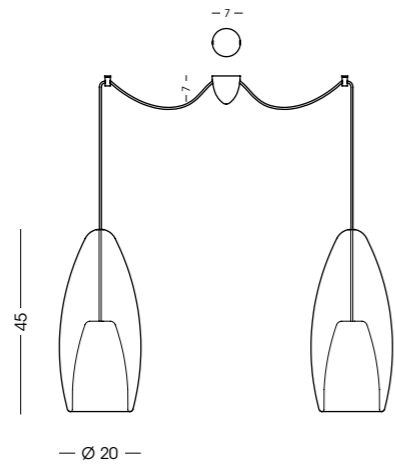
XXL1393.2L Sospensione / Hanging lamp vetro/glass Ø20 cm - cavo/cable 250 cm 2 E27 x max 105W 220-240V CE IP20 (1m)
