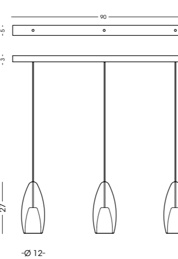
1397.90.3L Binario a soffitto / Ceiling track vetro/glass Ø12 cm - cavo/cable 150 cm 3 E14 x max 60W 220-240V CE IP20 (1m)
