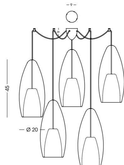
XXL1393.5L Sospensione / Hanging lamp vetro/glass Ø20 cm - cavo/cable 250 cm 5 E27 x max 105W 220-240V CE IP20 (1m)
