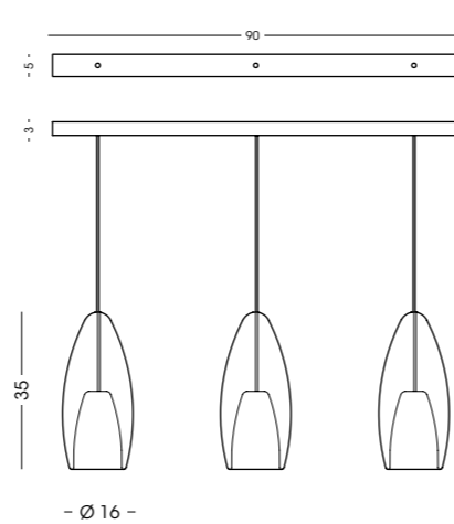
GIG1397.90.3L Binario a soffitto / Ceiling track vetro/glass Ø16 cm - cavo/cable 150 cm 3 E27 x max 105W 220-240V CE IP20 (1m)
