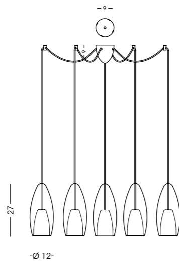
1393.5L Sospensione / Hanging lamp vetro/glass Ø12 cm - cavo/cable 250 cm 5 E14 x max 60W 220-240V CE IP20 (1m)
