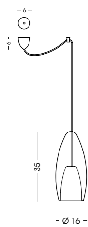
GIG1393.1LD Sospensione / Hanging lamp vetro/glass Ø16 cm - cavo/cable 250 cm 1 E27 x max 105W 220-240V CE IP20 (1m)
