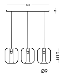
747.3L Binario a soffitto / Ceiling track vetro/glass Ø9 cm - cavo/cable 150 cm 3 G9 x max 42W 230V CE IP20 1m
