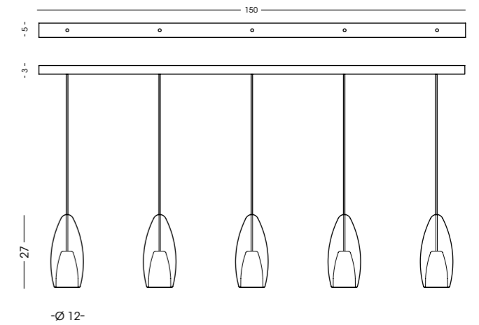
1397.150.5L Binario a soffitto / Ceiling track vetro/glass Ø12 cm - cavo/cable 150 cm 5 E14 x max 60W 220-240V CE IP20 (1m)
