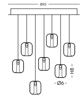
744.7L Plafoniera / Ceiling lamp vetro/glass Ø6 cm - cavo/cable 150 cm 7 G9 x max 42W 230V CE IP20 1m
