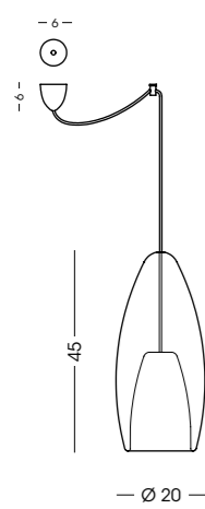
XXL1393.1LD Sospensione / Hanging lamp vetro/glass Ø20 cm - cavo/cable 250 cm 1 E27 x max 105W 220-240V CE IP20 (1m)
