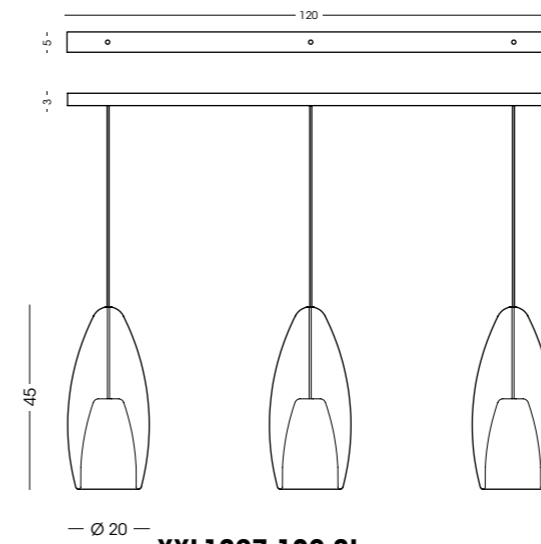
XXL1397.120.3L Binario a soffitto / Ceiling track vetro/glass Ø20 cm - cavo/cable 150 cm 3 E27 x max 105W 220-240V CE IP20 (1m)
