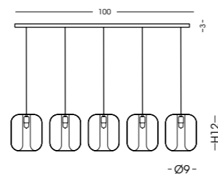
747.5L Binario a soffitto / Ceiling track vetro/glass Ø9 cm - cavo/cable 150 cm 5 G9 x max 42W 230V CE IP20 1m
