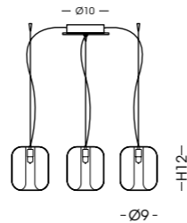
743.3L Sospensione / Hanging lamp vetro/glass Ø9 cm - cavo/cable 250 cm 3 G9 x max 42W 230V CE IP20 1m
