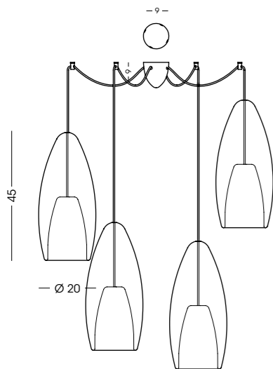
XXL1393.4L Sospensione / Hanging lamp vetro/glass Ø20 cm - cavo/cable 250 cm 4 E27 x max 105W 220-240V CE IP20 (1m)
