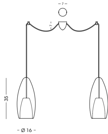
GIG1393.2L Sospensione / Hanging lamp vetro/glass Ø16 cm - cavo/cable 250 cm 2 E27 x max 105W 220-240V CE IP20 (1m)
