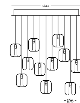
744.11L Plafoniera / Ceiling lamp vetro/glass Ø6 cm - cavo/cable 150 cm 11 G9 x max 42W 230V CE IP20 1m
