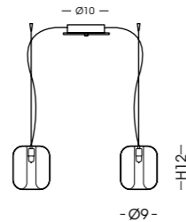
743.2L Sospensione / Hanging lamp vetro/glass Ø9 cm - cavo/cable 250 cm 2 G9 x max 42W 230V CE IP20 1m
