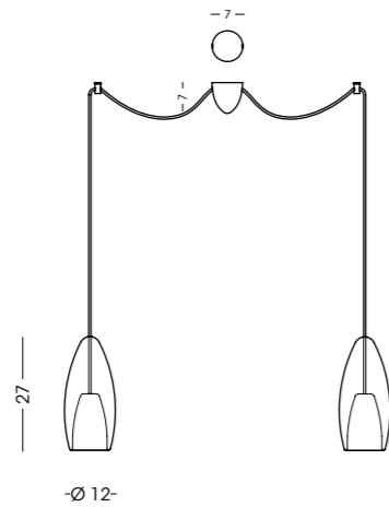
1393.2L Sospensione / Hanging lamp vetro/glass Ø12 cm - cavo/cable 250 cm 2 E14 x max 60W 220-240V CE IP20 (1m)
