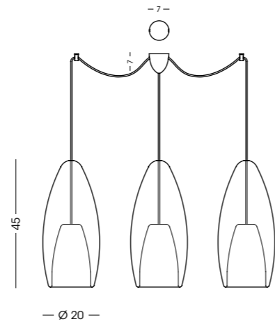
XXL1393.3L Sospensione / Hanging lamp vetro/glass Ø20 cm - cavo/cable 250 cm 3 E27 x max 105W 220-240V CE IP20 (1m)
