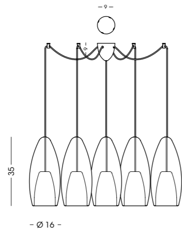
GIG1393.5L Sospensione / Hanging lamp vetro/glass Ø16 cm - cavo/cable 250 cm 5 E27 x max 105W 220-240V CE IP20 (1m)
