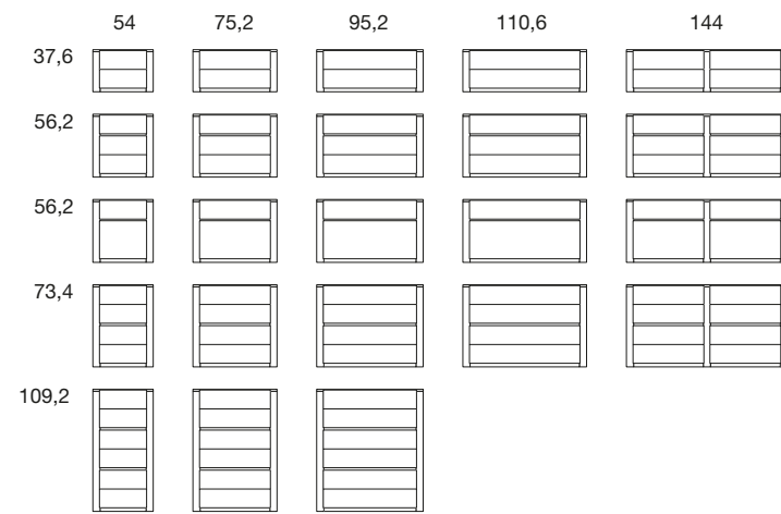
CASSETTIERE PROF. 50 DRAWER UNIT DEPTH 50
