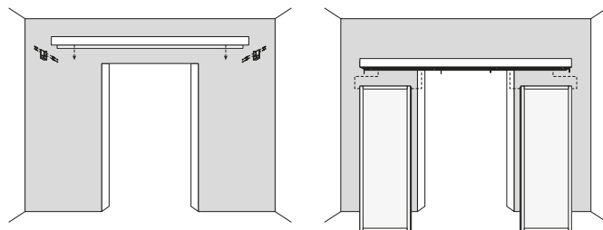
FISSAGGIO BINARIO A 1 VIA A PARETE 1-WAY RAIL TO WALL FIXING
