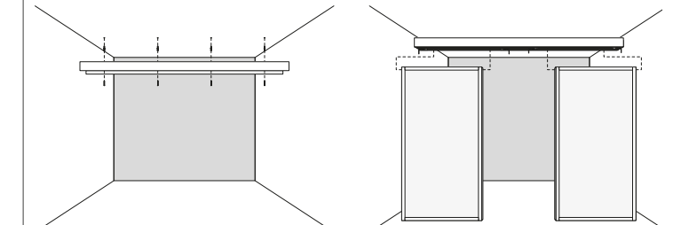
FISSAGGIO BINARIO A 2 VIE A SOFFITTO 2-WAY RAIL TO CEILING FIXING
