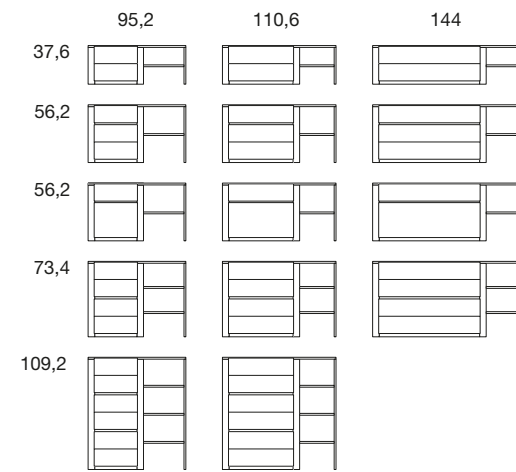
CASSETTIERE CON VANI A GIORNO PROF. 50 DRAWER UNIT WITH OPEN COMPARTMENTS DEPTH 50
